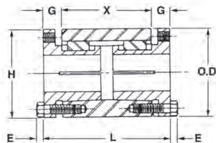
Type CSP and CSQ
