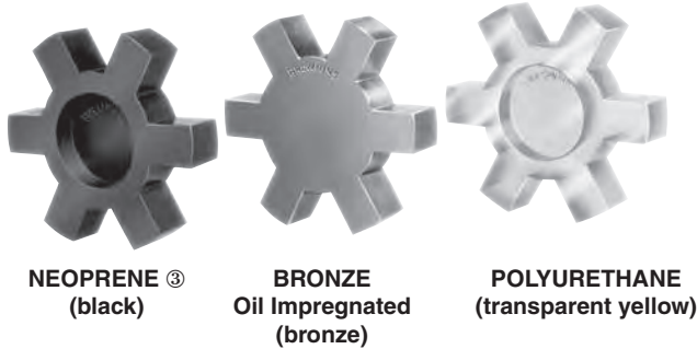
Jaw Coupling Inserts
