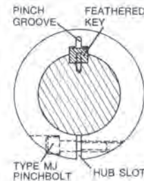
Section View of Type MJ Slide Hub on a Shaft
