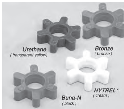
Type L Jaw Couplings offer a choice of four insert materials.
