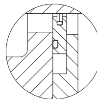
Piston Spirolox* Seal Ring
