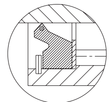
Lip Seal
